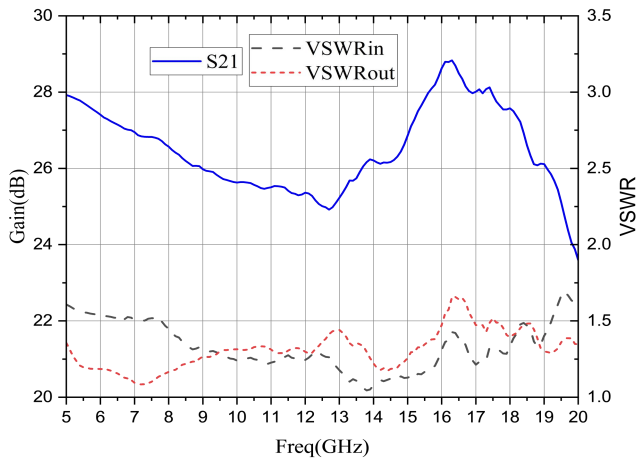
Gain & VSWR(IN&OUT)
