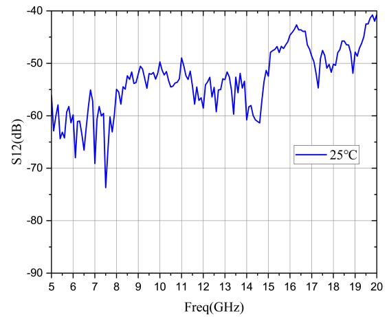
Reverse Isolation
