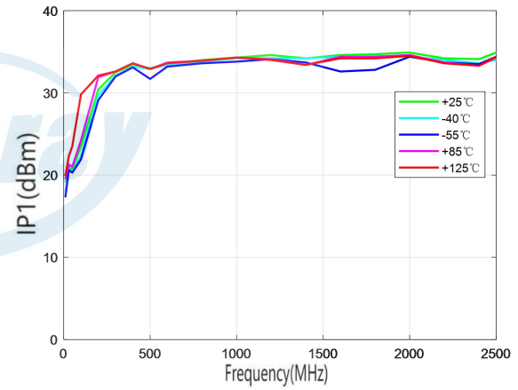
Input Power for 1dB Compression
